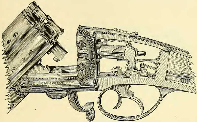
Lancaster Four-barrelled Gun.
